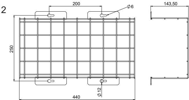
62858 - PROTECTIVE CAGE
