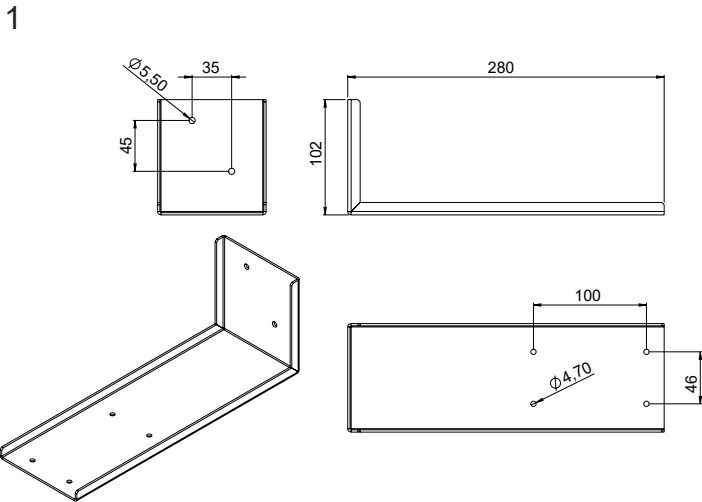
6902 - Wall bracket
