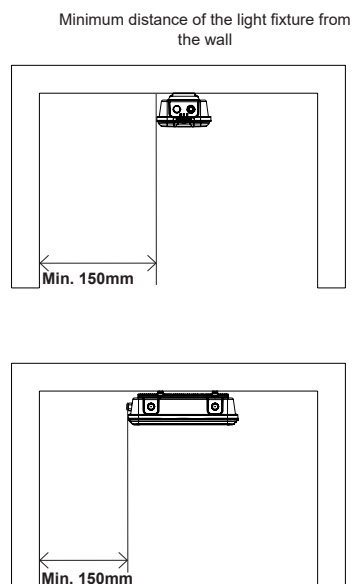
Picture. 5 Conditions of outdoor assembly
