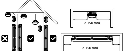
Outdoor installation conditions Fig. 7
