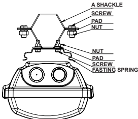
Outdoor installation conditions Fig. 7
