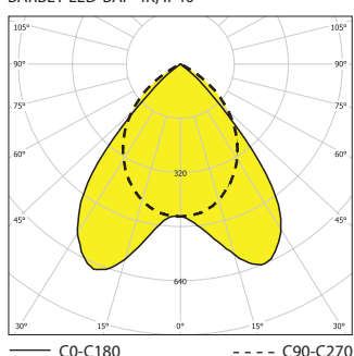
BARBET-LED-BAP-4K, IP40
